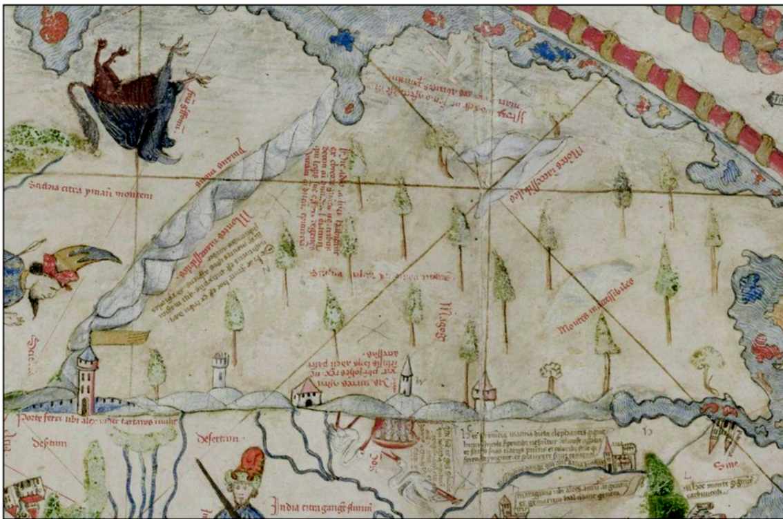
Detail of so-called Genoese World Map: Region enclosed by Alexander (Magog) (#248)
